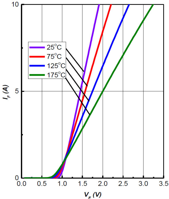
Figure 1. Forward Characteristics
