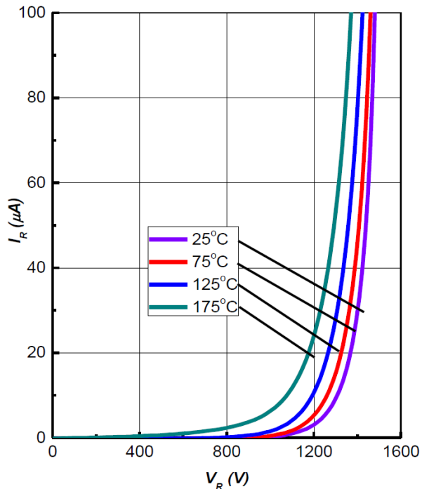
Figure 2. Reverse Characteristics
