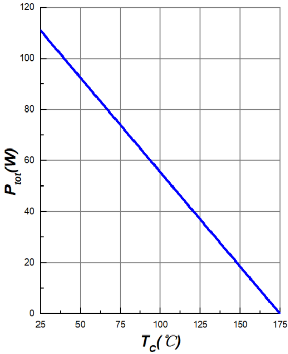
Figure 3. Power Derating
